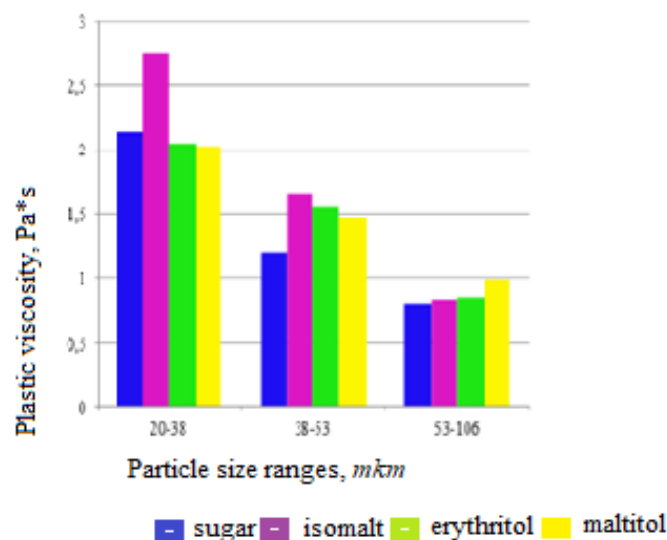
Fig. 1. Plastic viscosity of chocolate samples in different particle size ranges
